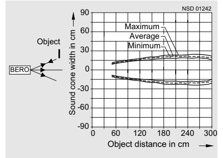
Measurement 3 (plane object), attenuation 4
