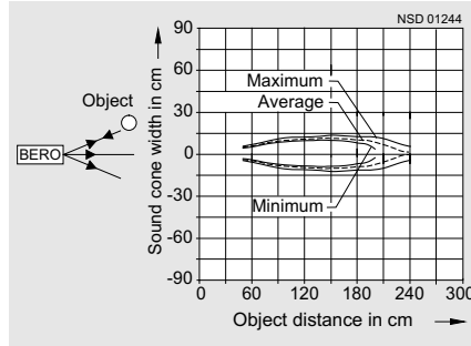
Measurement 2 (cylindrical object), attenuation 6
