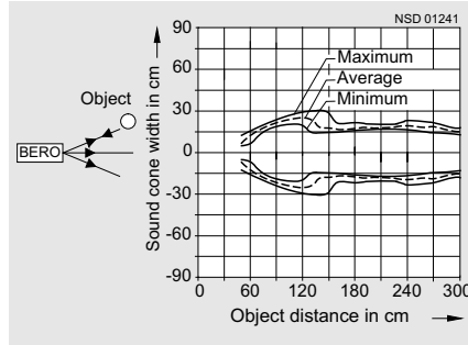
Measurement 2 (cylindrical object), attenuation 4
