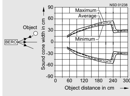
Measurement 2 (cylindrical object), attenuation 2
