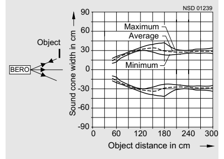
Measurement 3 (plane object), attenuation 2
