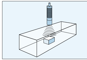
Object measurement: M18 compact range with switching output
